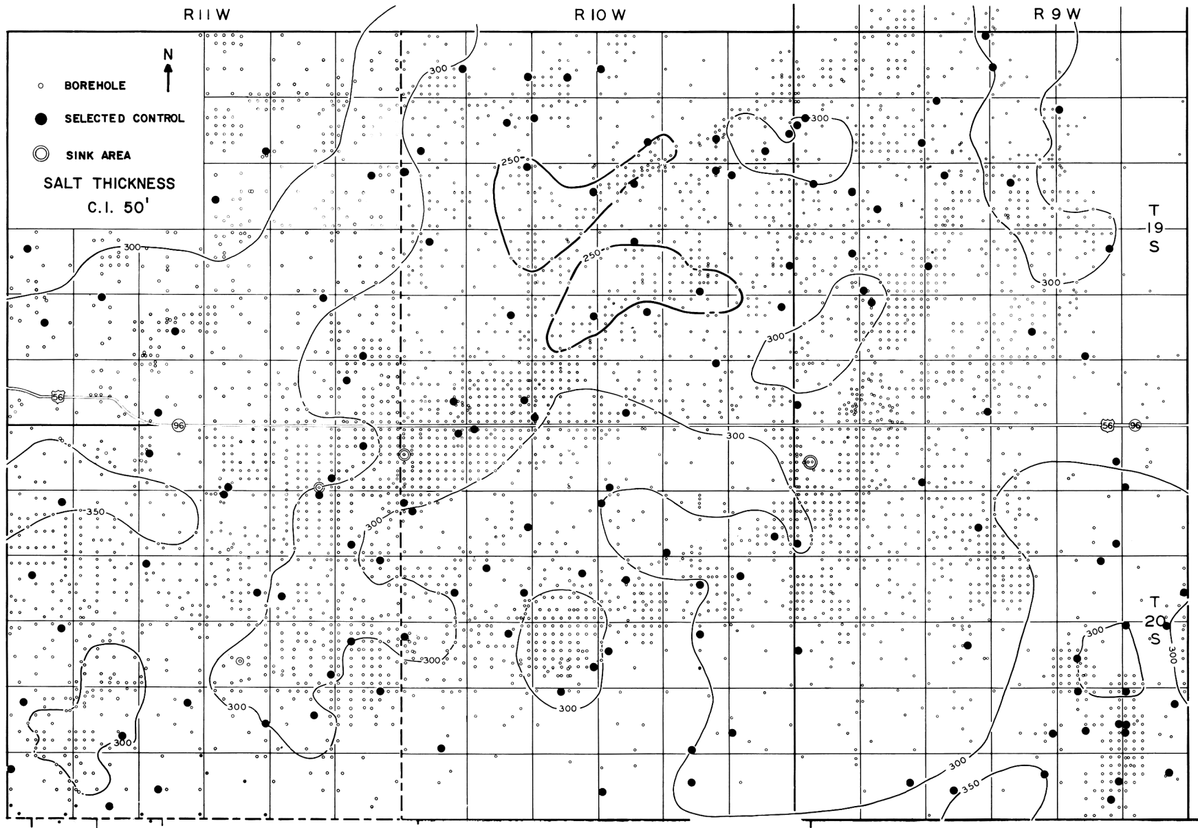
Figure 26--Map: thickness of salt, Chase-Silica Oil Field. Contour interval 50 feet.
