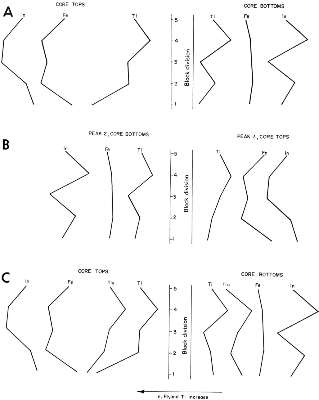
FIGURE 25.—Lateral variation comparison graphs of insoluble residue (In) content and iron (Fe) content with thermoluminescence (TI) of A , peak 1; B , peak 2 and peak 3; and C , peak 4 and peak 4u (Tlu).
