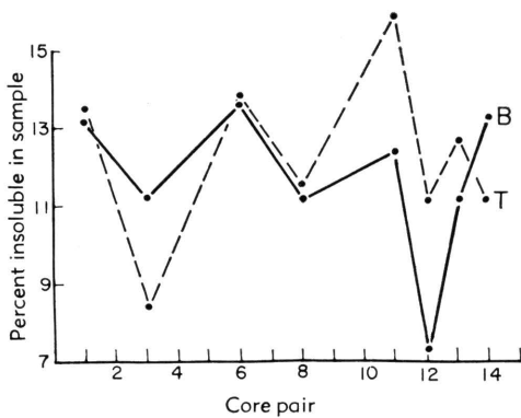
FIGURE 23.—Insoluble residue content vertical variation comparison graph.
