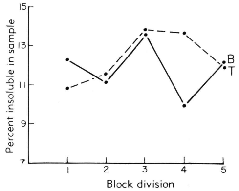
FIGURE 24.—Insoluble residue content lateral variation comparison graph.
