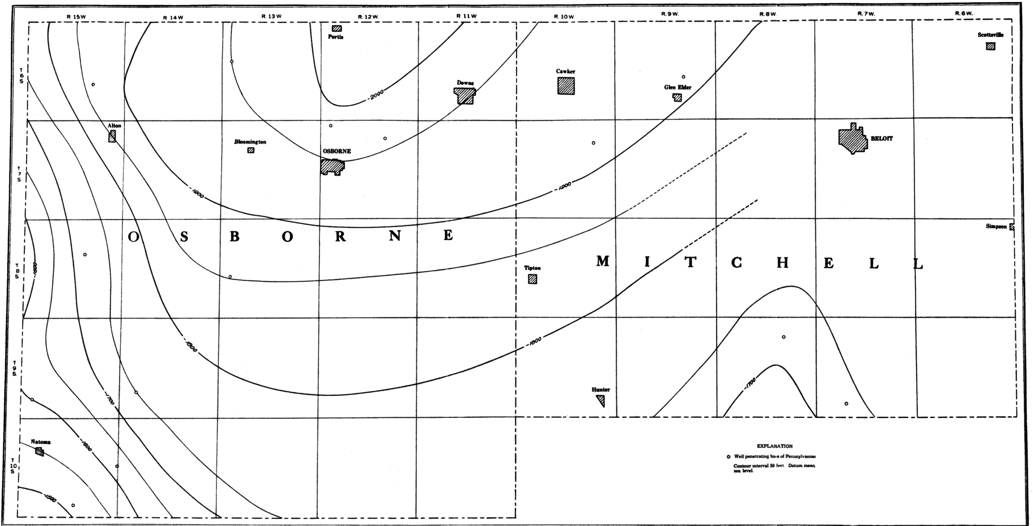
PLATE XIII.—Structural contour map of base of Pennsylvanian, Osborne and Mitchell counties.
