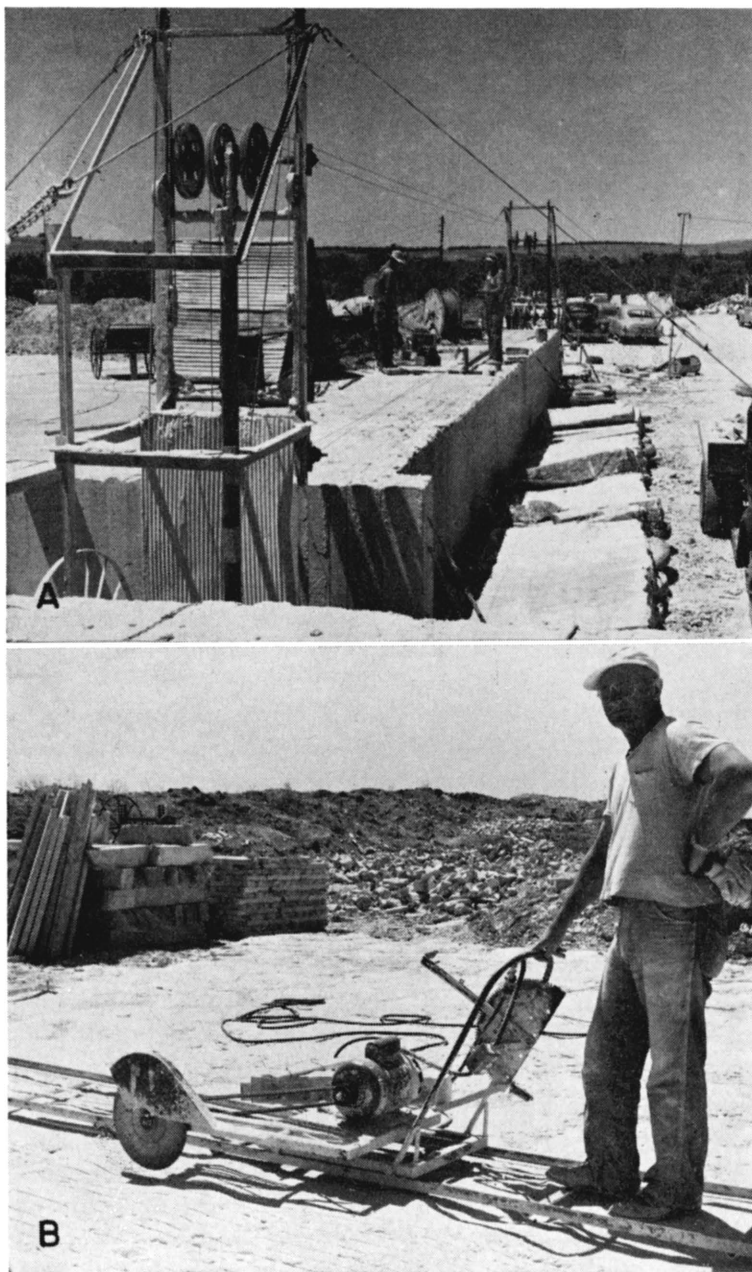
PLATE 2.— A , Junction City Stone Company Quarry. Multiple wire saw cutting slabs of Fort Riley Limestone. B , Sawing direct-cut strips of "shell rock" in Simpson Limestone Quarry, near Simpson.
