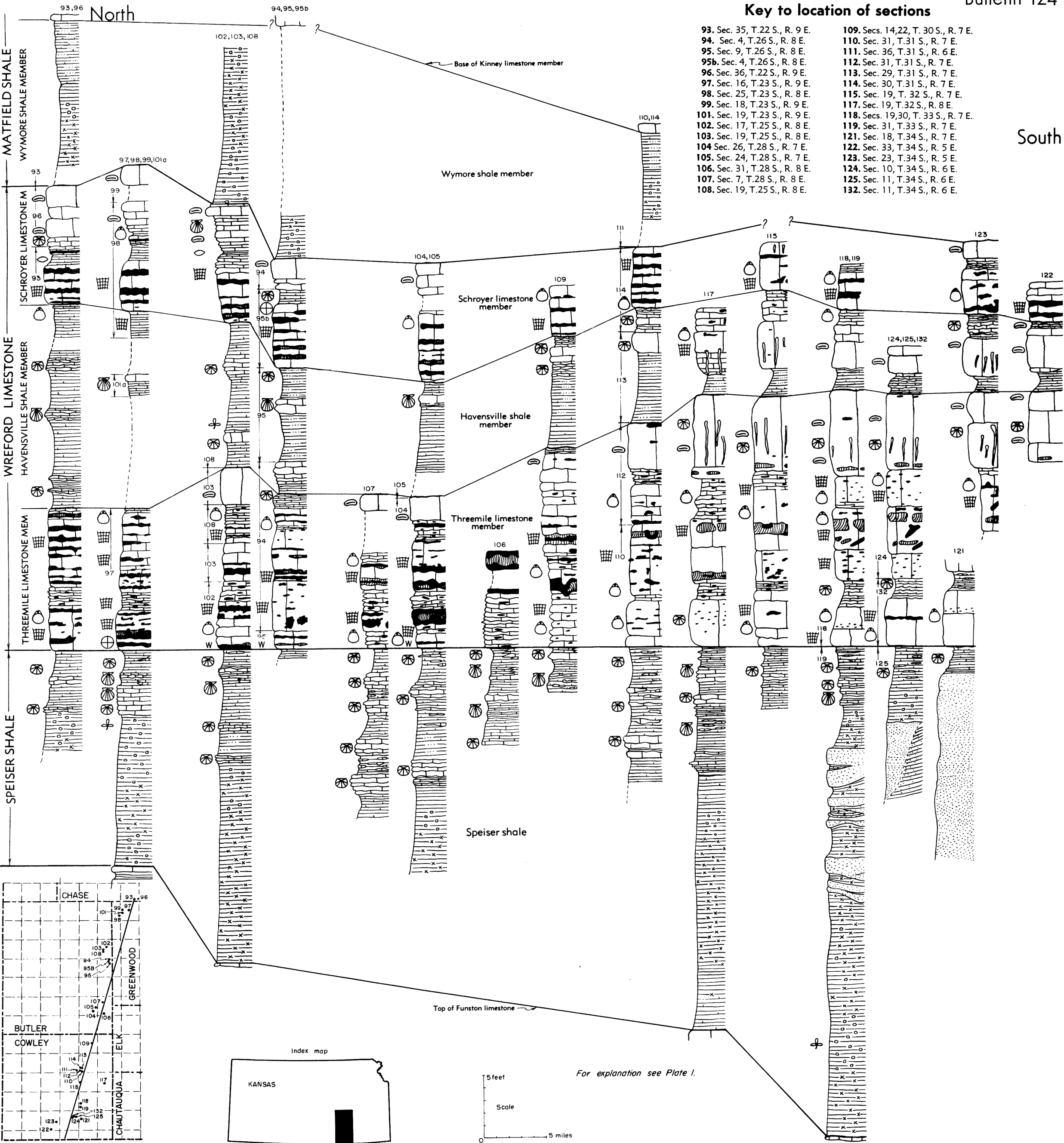
Plate 3. CORRELATION OF THE WREFORD MEGACYCLOTHEM By Donald E. Hattin, 1954
