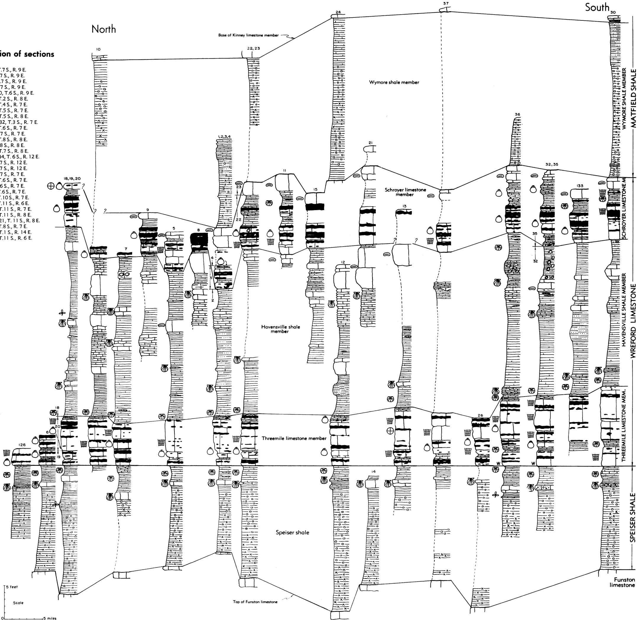
Plate 1. CORRELATION OF THE WREFORD MEGACYCLOTHEM
