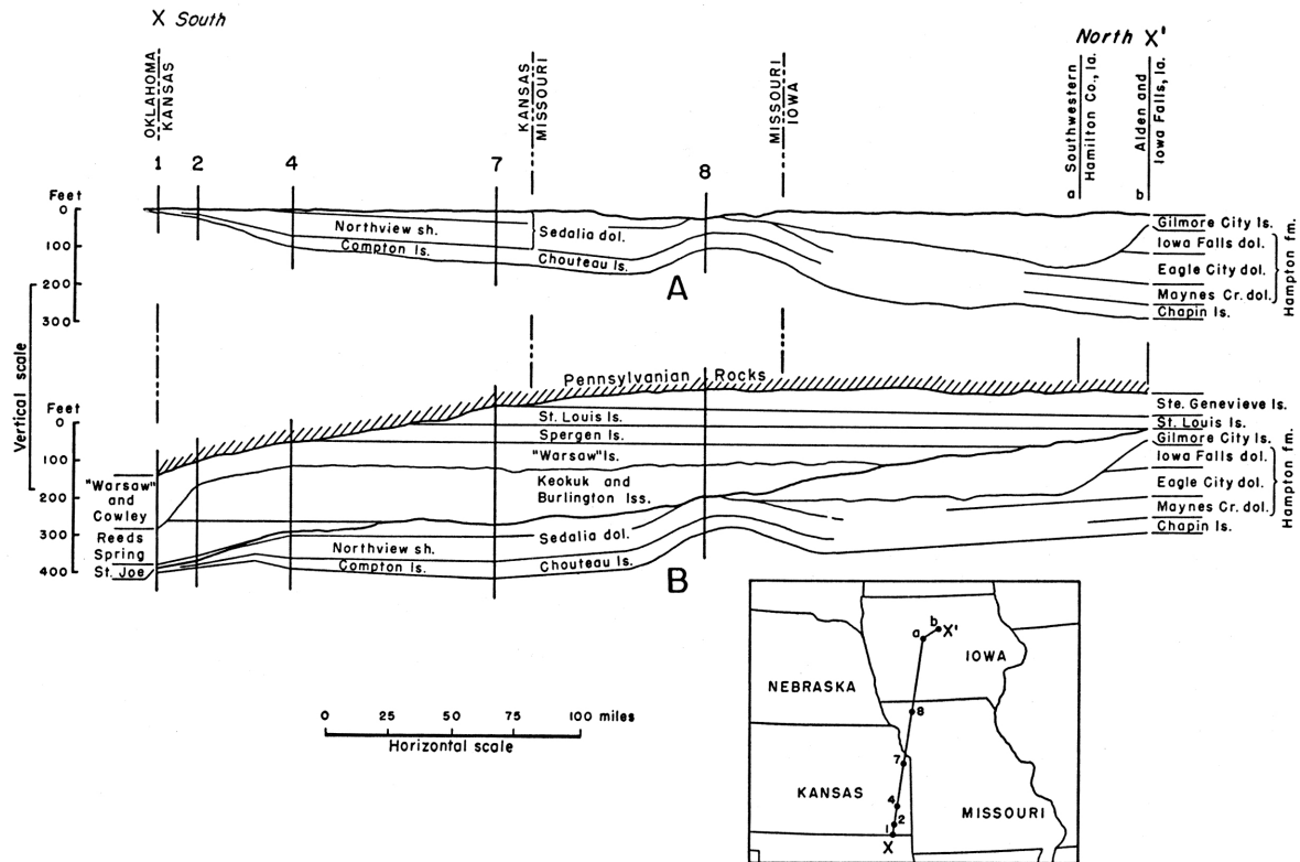
FIG. 20.—Diagrammatic cross sections from southeastern Kansas to central Iowa, showing northerly thickening of Kinderhookian limestones and northerly thinning and overlap of younger Mississippian formations. Compare with Figure 13.
