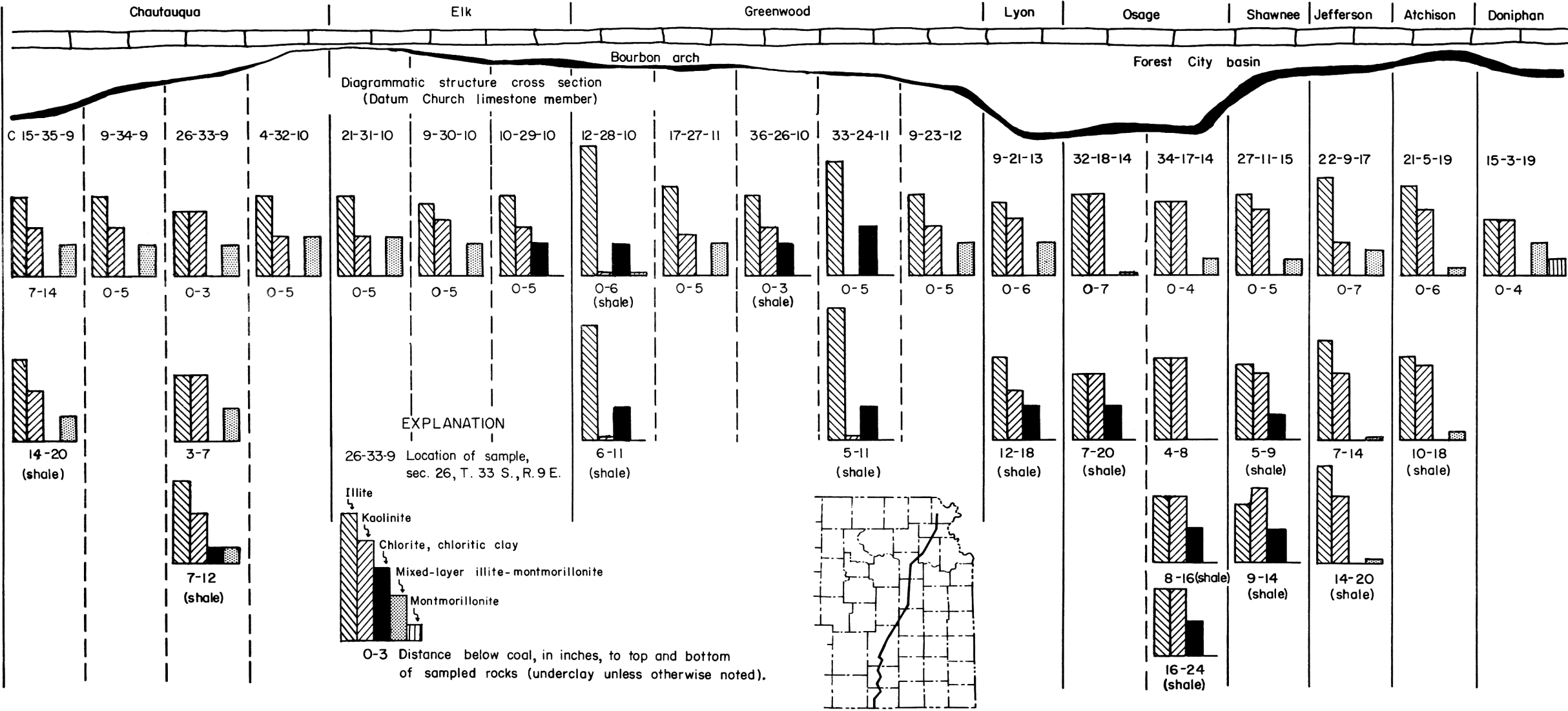
Estimated Amounts of Clay Constituents in Nodaway Underclay and Underlying Shale, and Relationship to Structure
