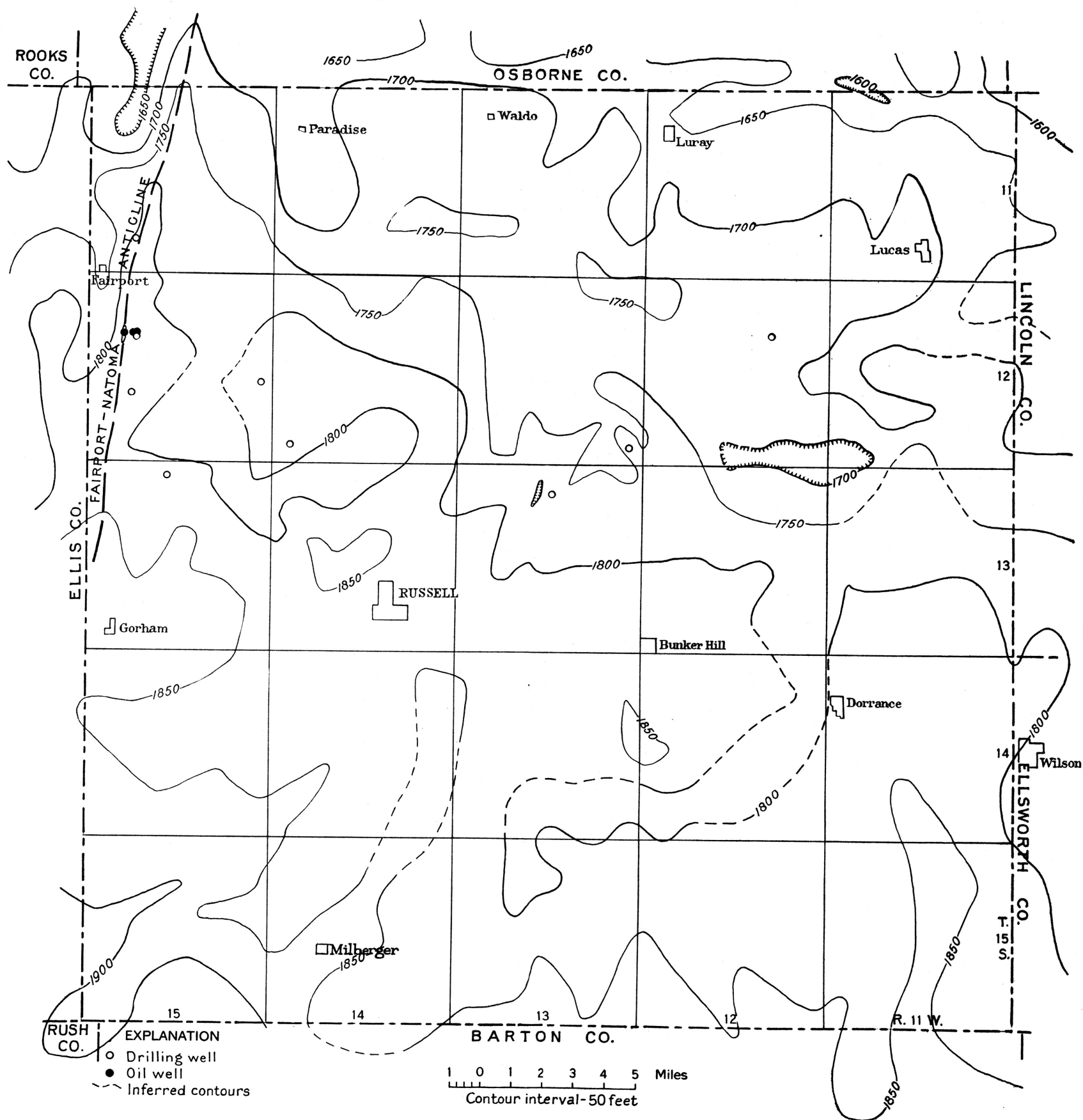
Generalized structural contour map of Russell county, Kansas. Elevations on upper surface of Greenhorn limestone—the top of the “fence-post limestone.”
