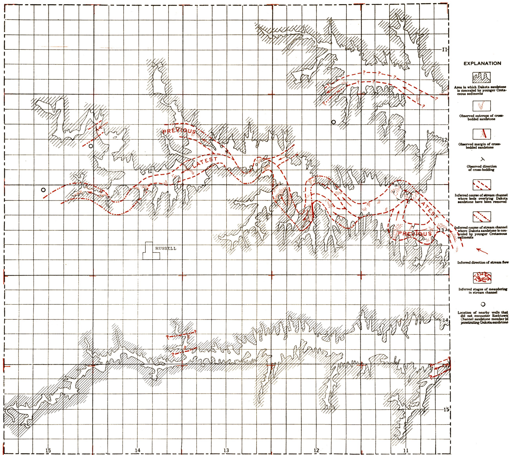
Approximate location in the Dakota area of Russell county of meander belt of stream and tributaries (?) that deposited the Rocktown channel sandstone member of the Dakota sandstone.
