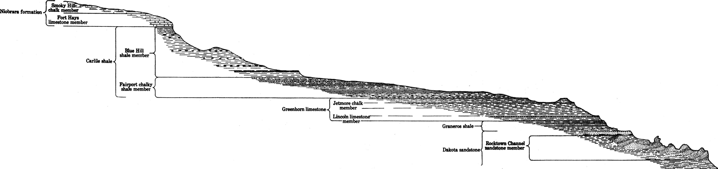
A. Idealized profile through the Cretaceous strata of Russell county, Kansas.
