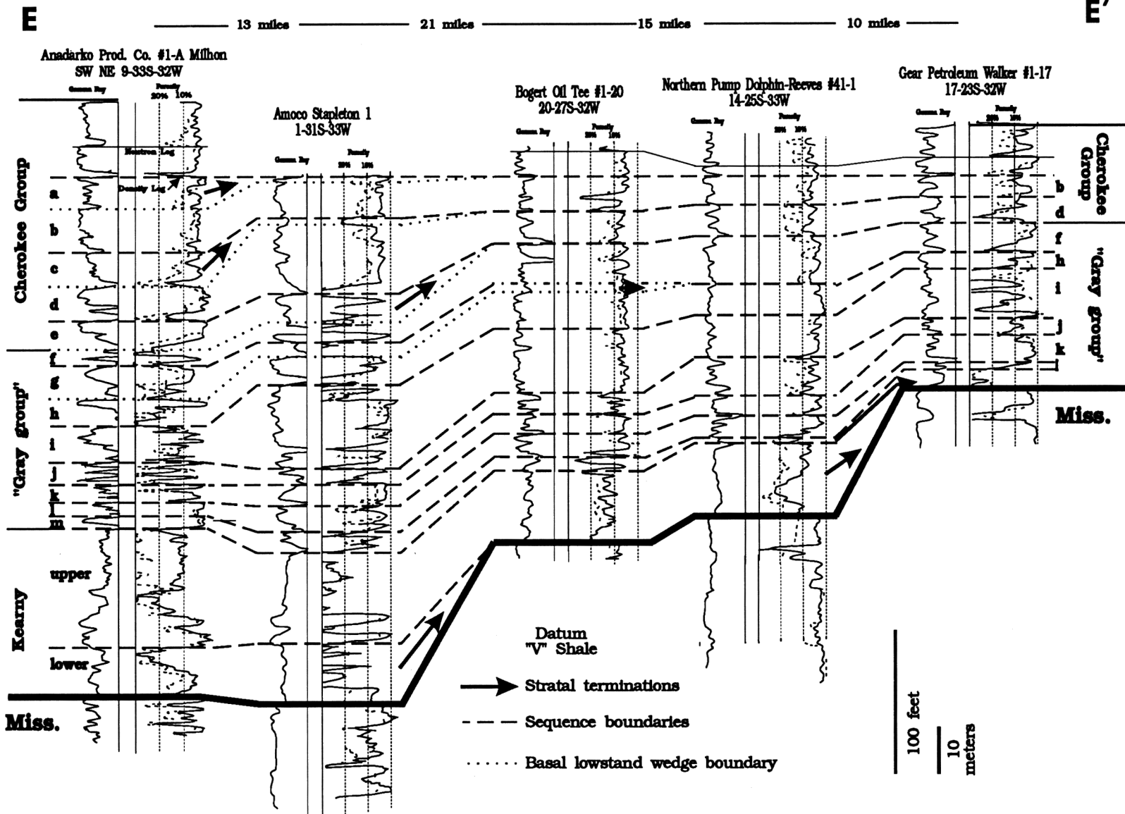
FIGURE 6—CROSS SECTION E-E' FROM EAST-CENTRAL SEWARD COUNTY NORTH THROUGH FINNEY COUNTY.
