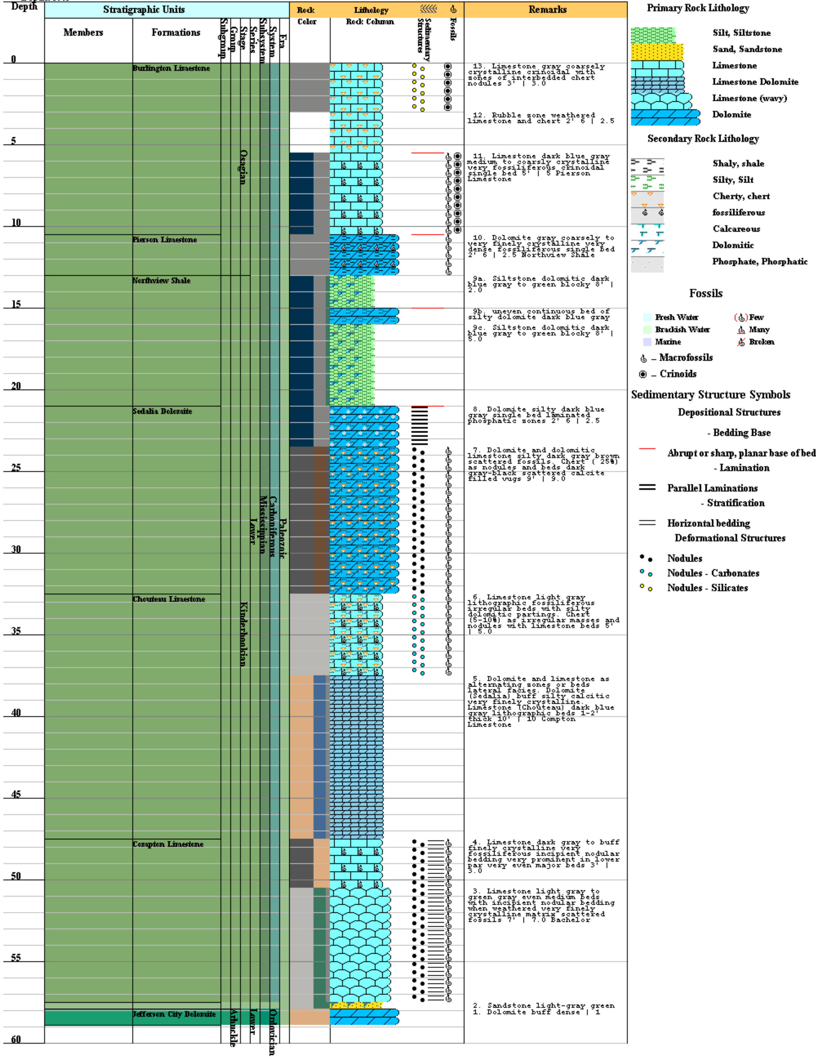
Figure 28 Mississippian System (RI 70) - Kinderhookian T: 47N R: 21W S: 33 Depth: 59.0
