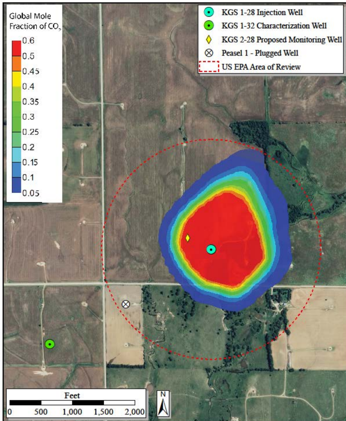
Figure ES-5b Maximum lateral extent of CO 2 plume migration.
