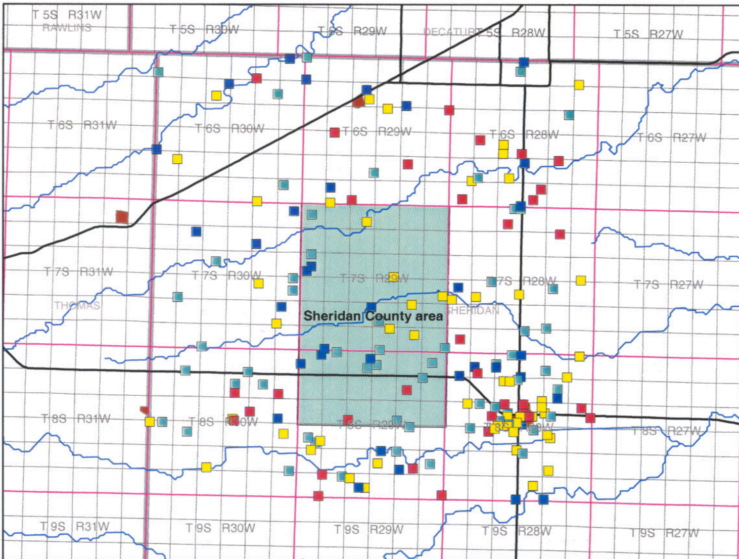
Figure 30 1 The coarse fraction percentiles in the lower half of the combined Ogallala Formation – undifferentiated Quaternary, Sheridan County study area. Drawn by Date File Name Projection Scale grh 02/10/03 Fig 30 Coarse frac L.mxd UTM Zone 14 NAD 1983 1:250,000
