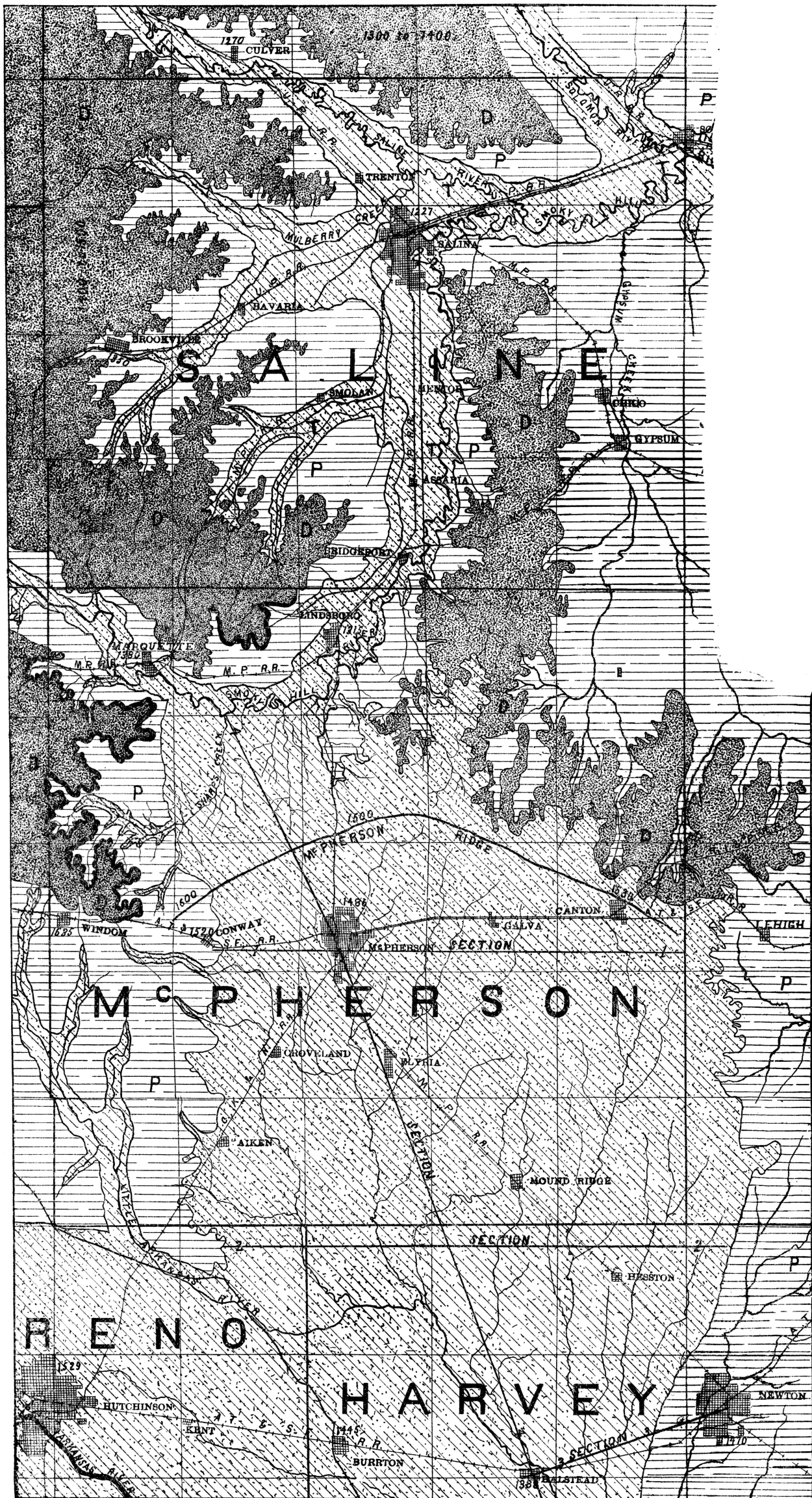
GEOLOGIC MAP OF McPHERSON AND VICINITY. By C. S. Prosser and J. W. Beede.
