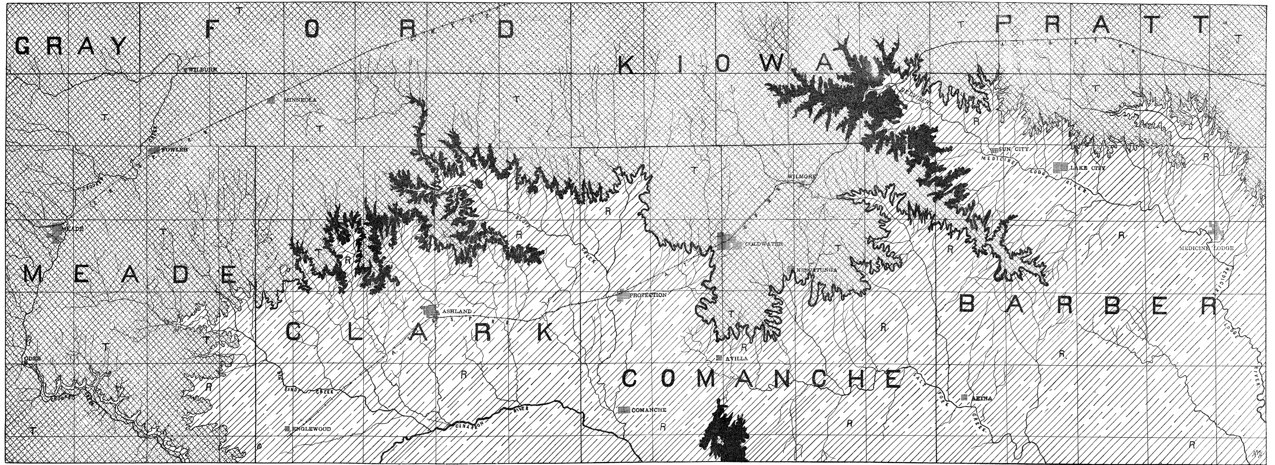
A GEOLOGIC MAP OF SOUTHWEST COMANCHE AREA. By CHARLES S. PROSSER.
