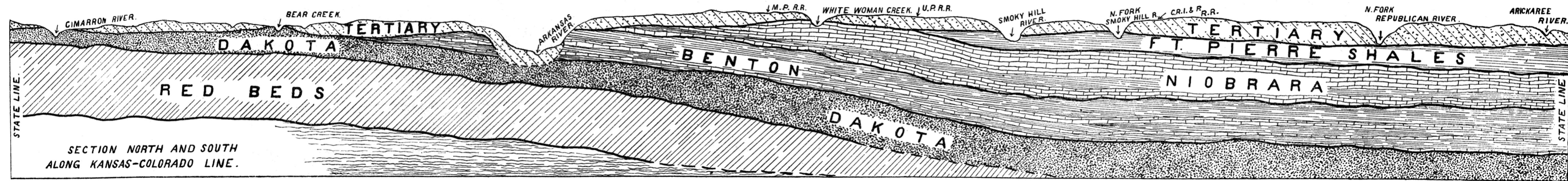
A GEOLOGIC CROSS SECTION FROM NORTH TO SOUTH ALONG THE WEST END OF KANSAS, SHOWING RELATIONS OF DIFFERENT FORMATIONS TO EACH OTHER.
