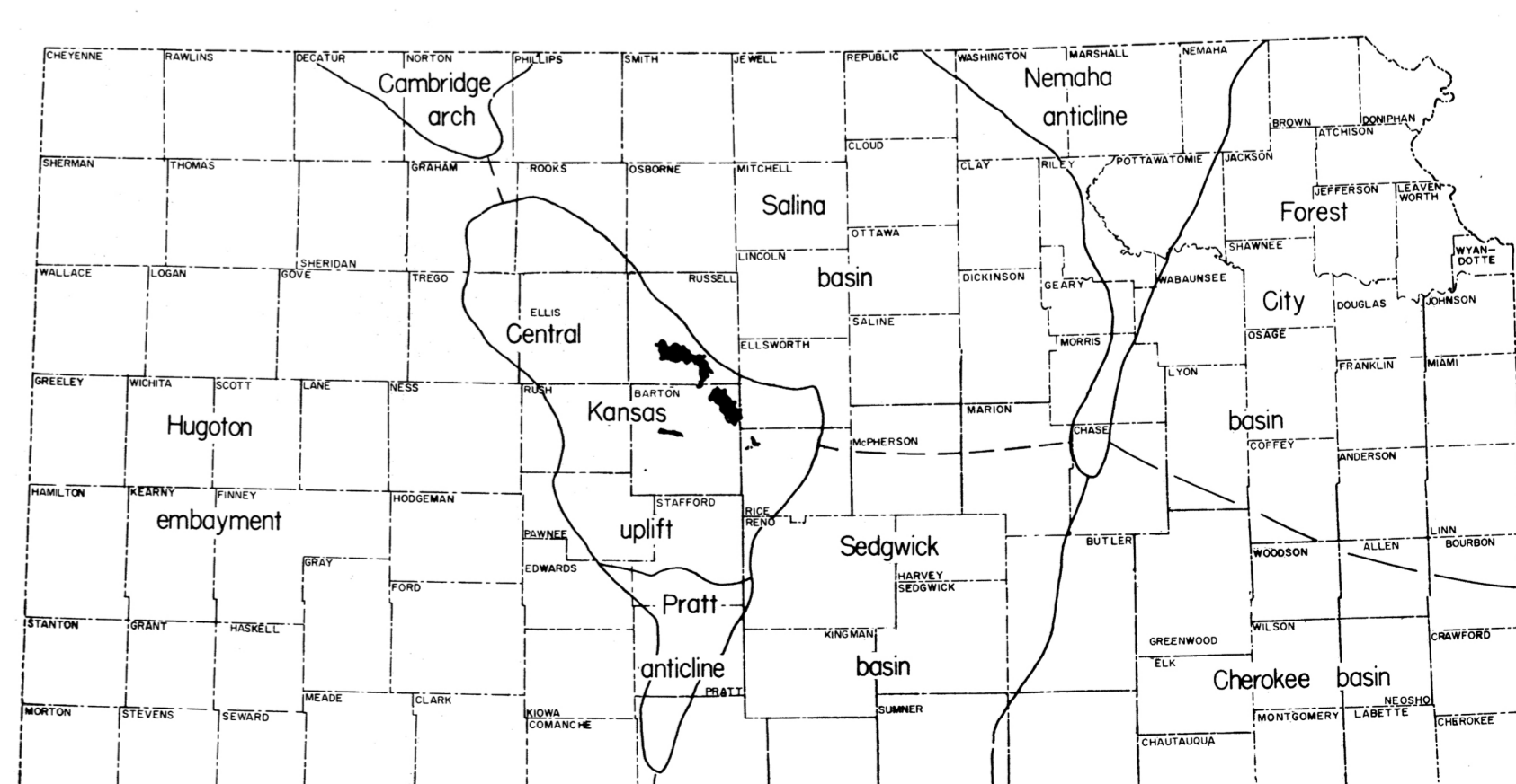
Precambrian
