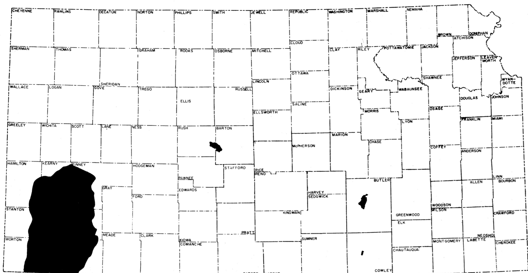
Lower Permian
