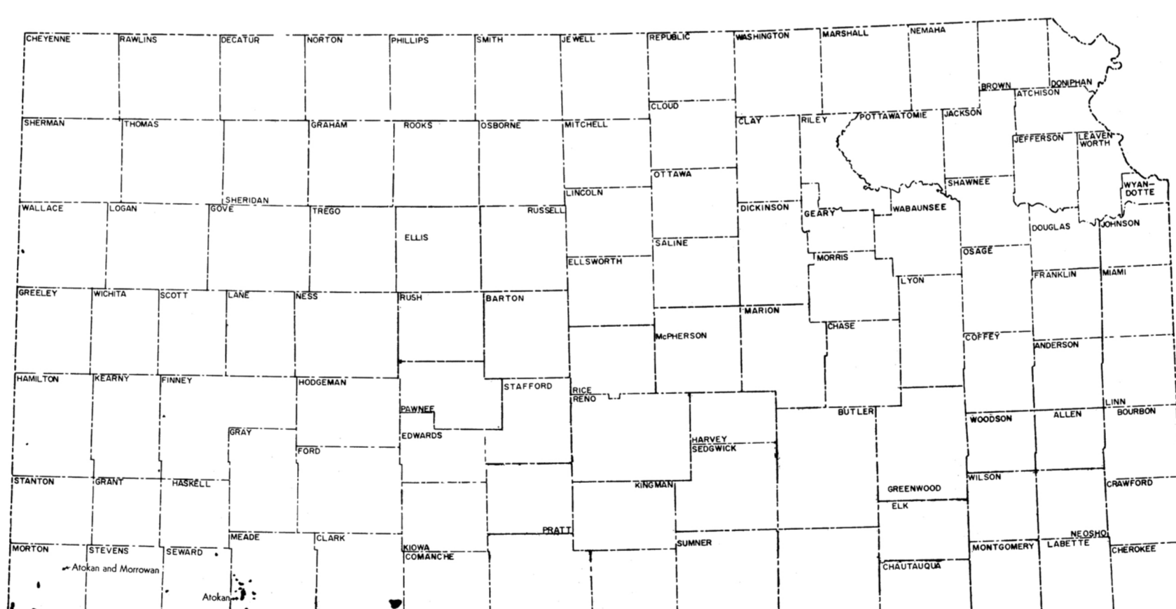
Atokan and Morrowan (all fields Morrowan except where otherwise indicated)
