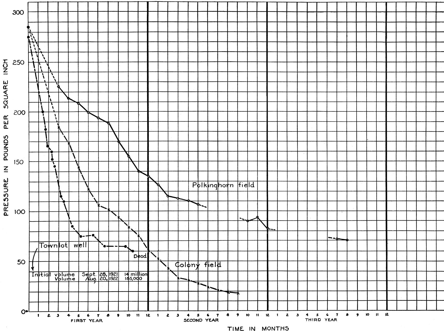
PLATE VIII.—Pressure decline curves of the Colony townsite field and the Polkinghorn field. The latter curve is included in the same graph to allow comparison of the decline of fields in which the wells were located at different distances from each other. The townlot well was on the 40-acre tract that held 31 gassers.
