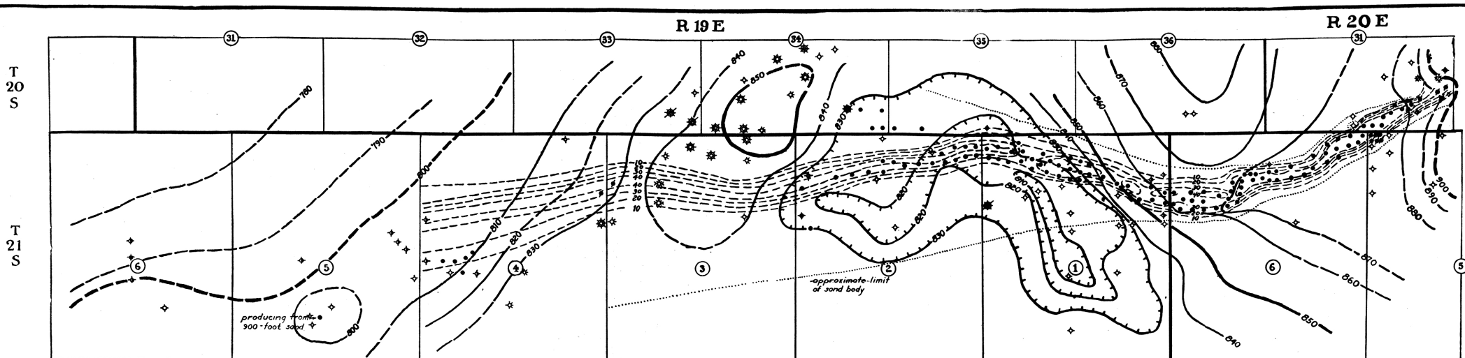
SAND THICKNESS AND STRUCTURAL MAP
