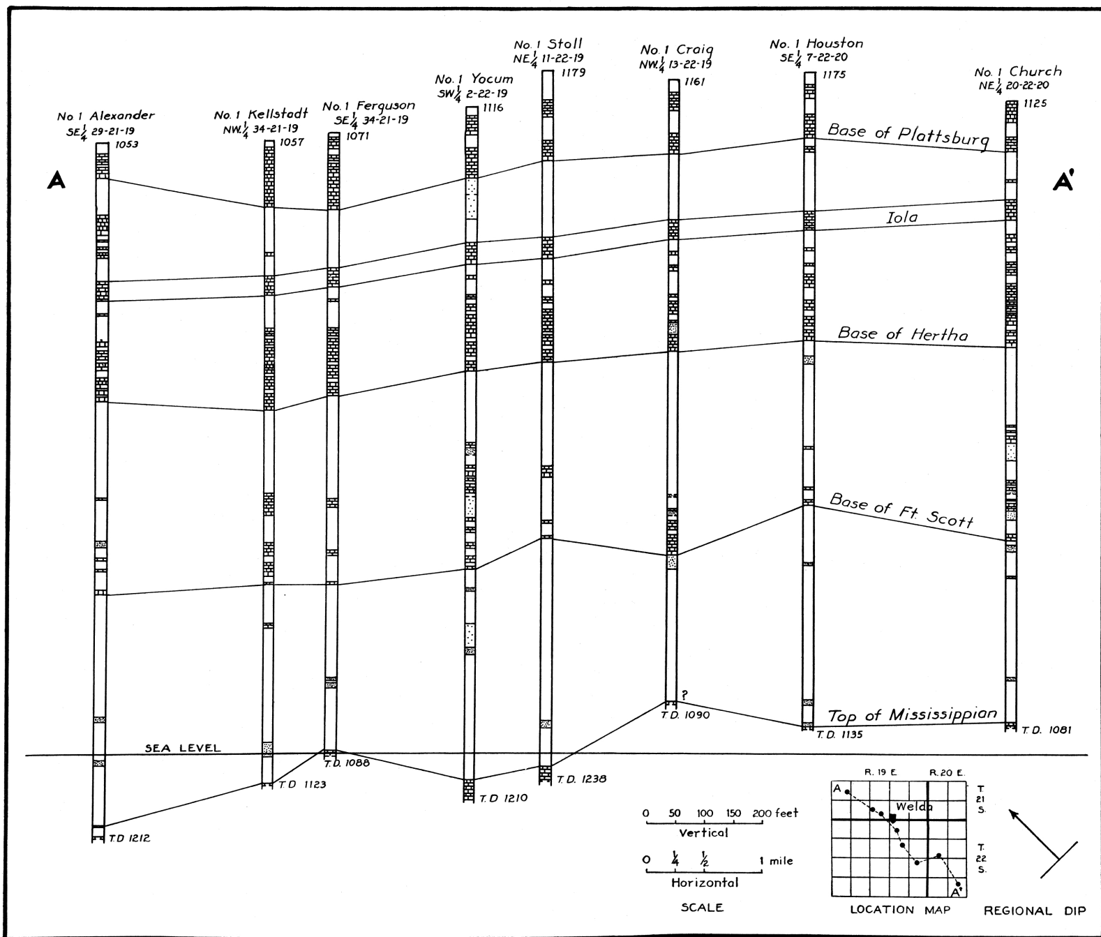
PLATE III.—A section to show the lack of effect on the attitude of the Pennsylvanian sediments of gravitational compaction over the Mississippian rocks. This section also demonstrates the inaccuracy of the parts of the well logs that include the thin limestones of the Marmaton formation.
