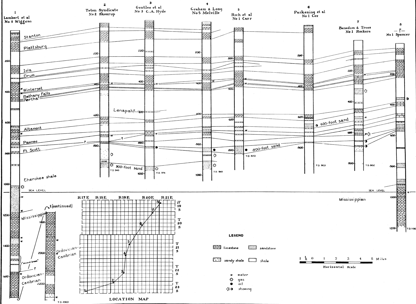
PLATE II.—Northeast-southwest geological cross section of Anderson county.
