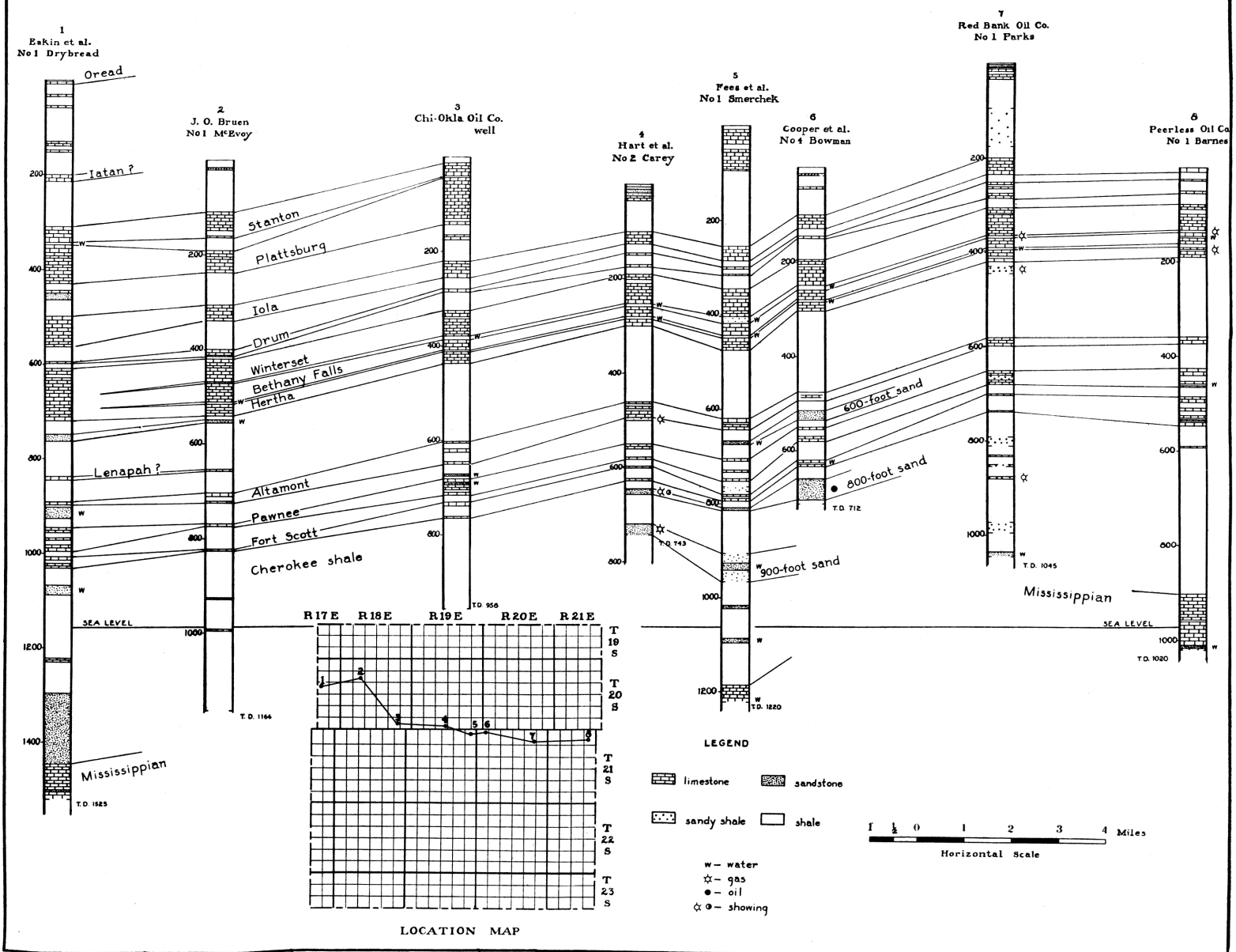
PLATE I.—East-west geological cross section of Anderson county.
