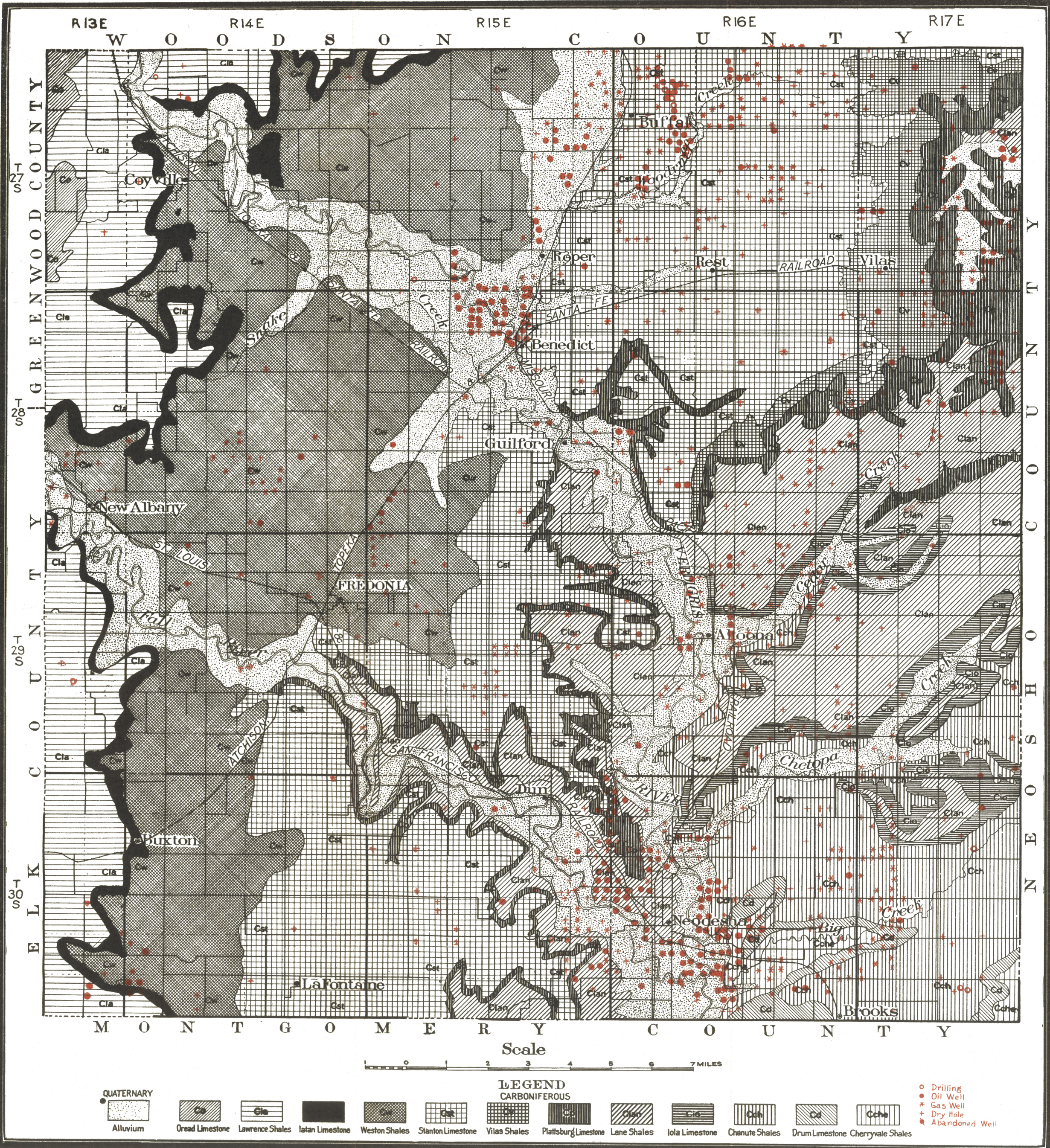
Geologic map of Wilson county, showing location of oil and gas wells. (Geology after Haworth and Bennett.)
