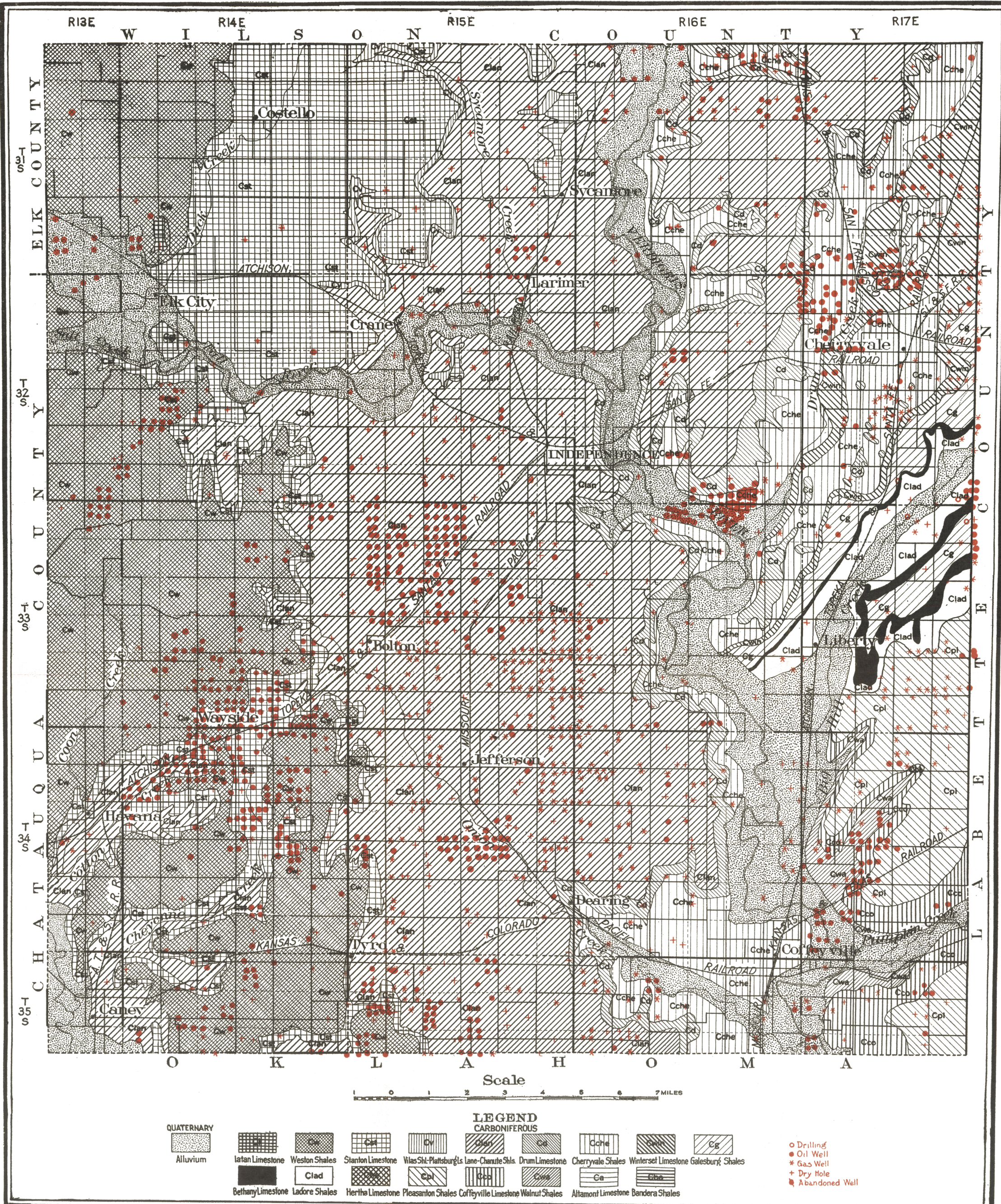
Geologic map of Montgomery county, showing location of oil and gas wells. (Geology after Haworth and Bennett.)
