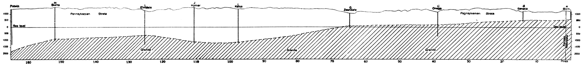
A. Geologic section along granite ridge from Bern, Neb., to Potwin, Kan., showing top of granite.
