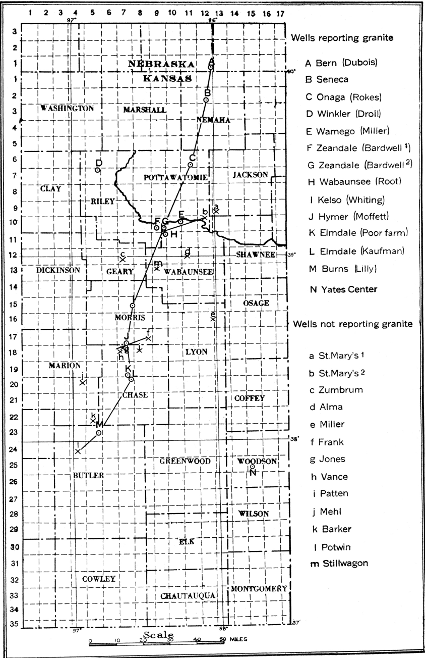
Location map of central Kansas, showing wells which have encountered granite and associated wells which have not reached granite. The lines of sections A, B, C, Plate XXII, are shown.
