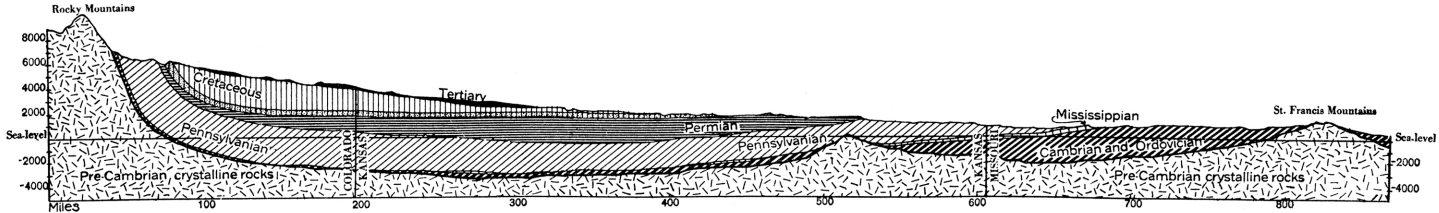
Geologic cross-section in an east-west direction across the Kansas region.
