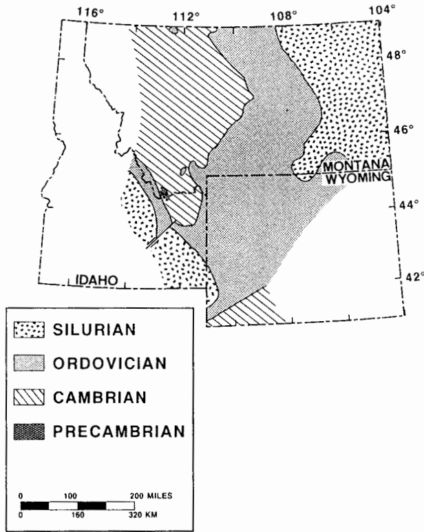
Figure 2. Pre-Devonian paleogeologic map. Modified from Sandberg and Mapel (1967) and Baars (1972) using data from Churkin (1962) and Scholten (1957, 1960) and unpublished field data. Note that the oldest rocks beneath Devonian deposits are located in southwestern Montana near the present Montana–Idaho border. Lower Paleozoic subcrop patterns are highly generalized across the entire area.
