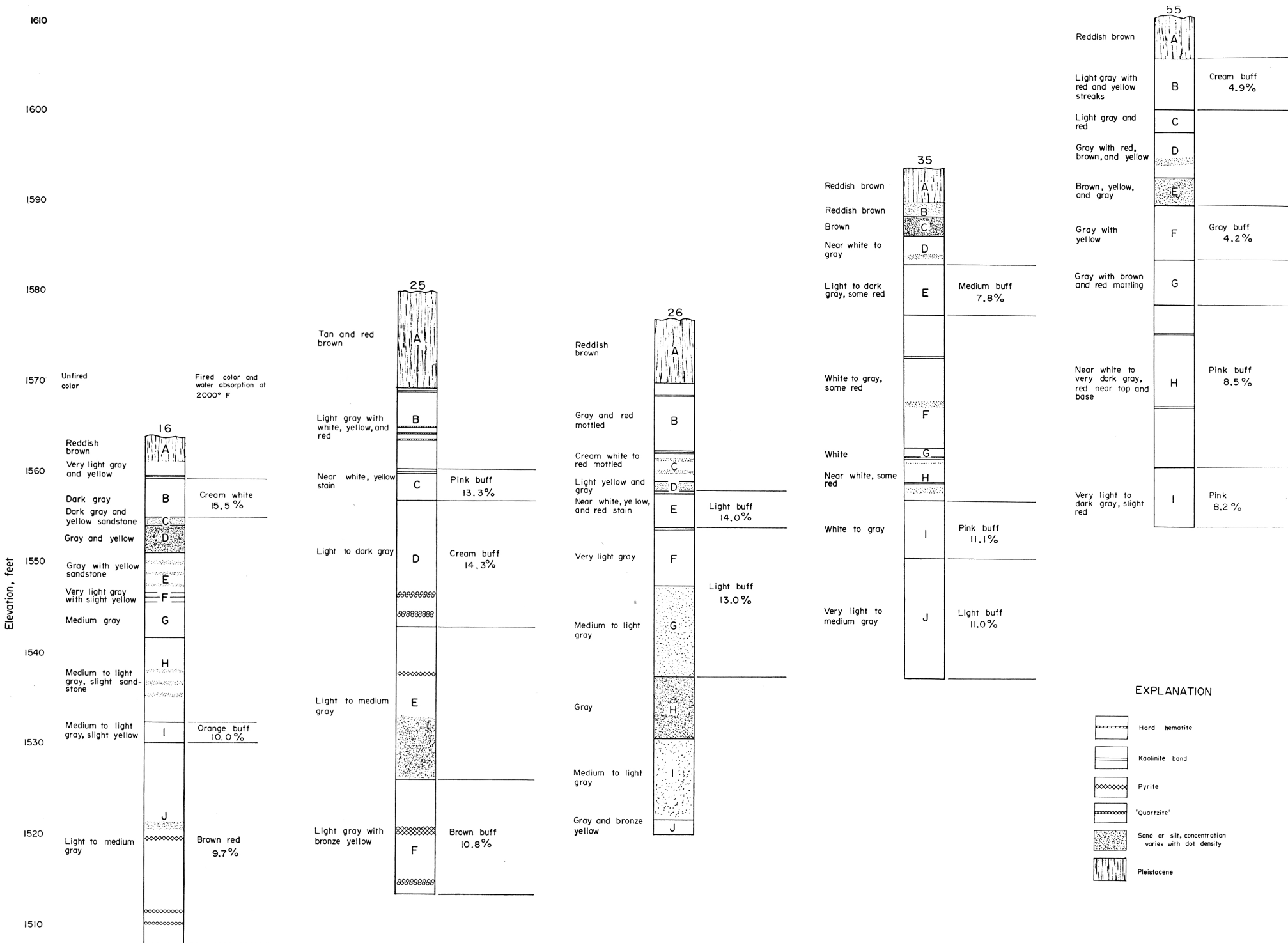
FIGURE 5.—Graphic logs of selected test holes in EL-14 area. (Locations of test holes shown on Figure 3; for test-hole numbers, see Appendix, Ellsworth County.)
