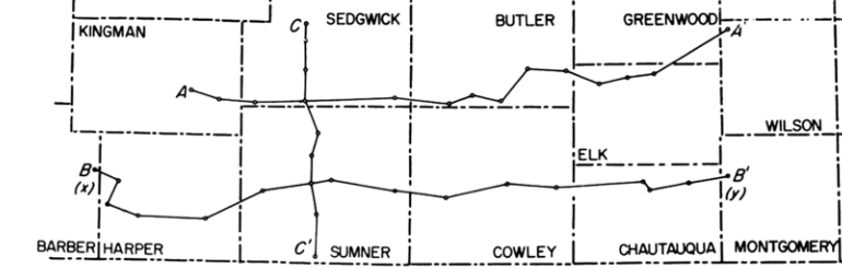
Index map showing location of cross sections
