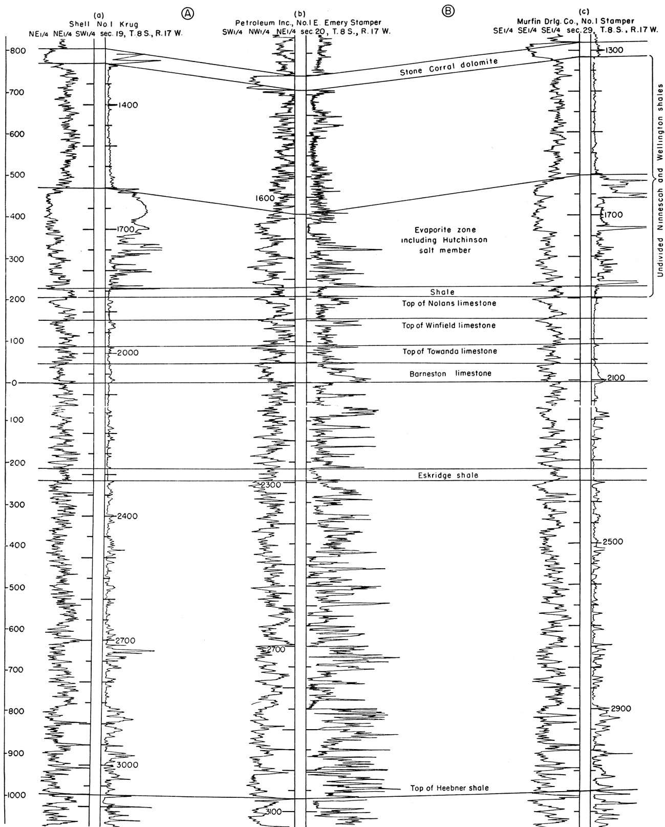
FIG. 17.—Correlation of electric logs (a), (b), and (c) of Figure 18 showing abrupt thickening of evaporite zone including Hutchinson salt member of Wellington formation.
