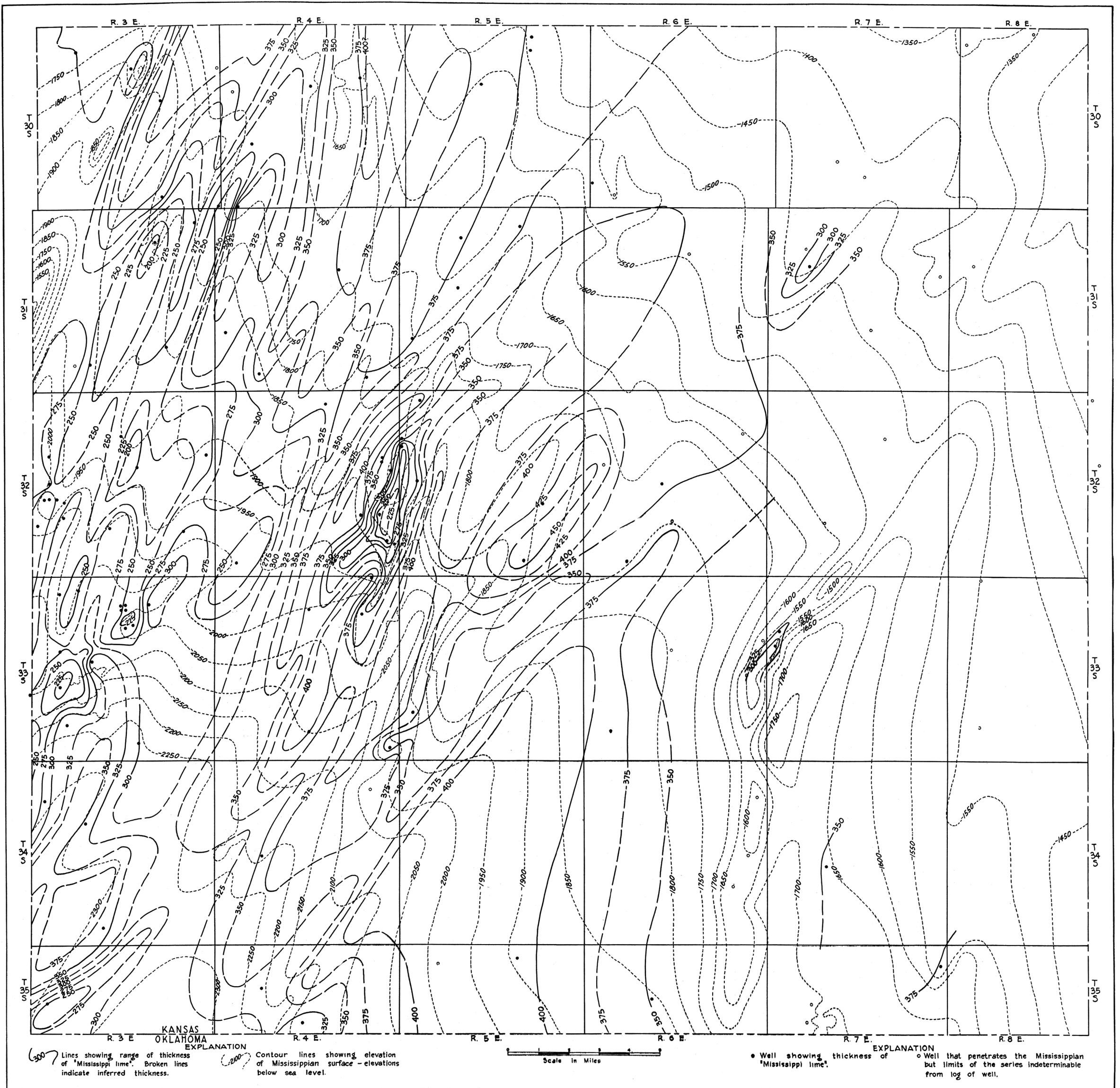
PLATE XII.—Sketch map showing thickness of the "Mississippi lime" and its relation to the attitude of the Mississippian surface in Cowley county.
