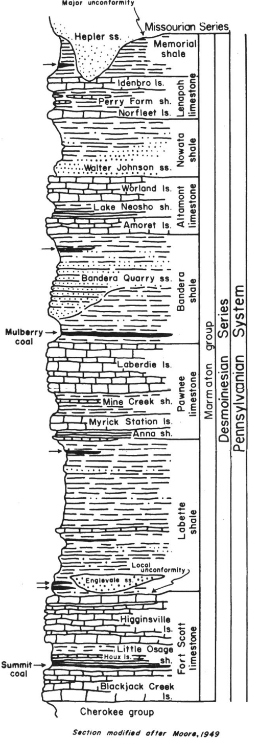
Generalized section of the Marmaton group of rocks in Kansas
