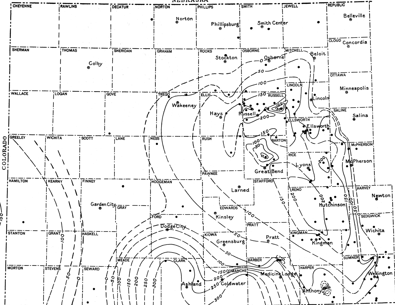
ISOPACHUS MAP SHOWING THICKNESS OF SALT IN WESTERN KANSAS
