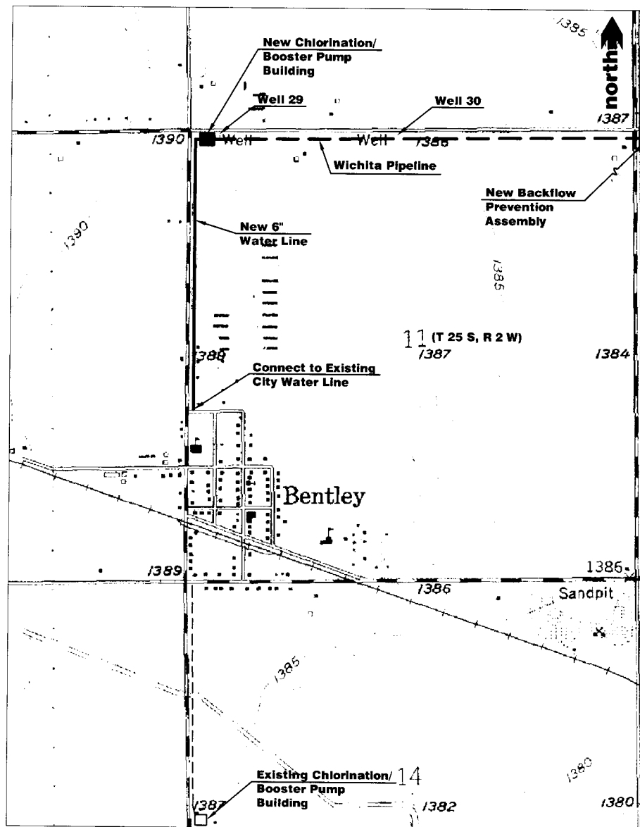
WATER SUPPLY IMPROVEMENTS BENTLEY, KANSAS
