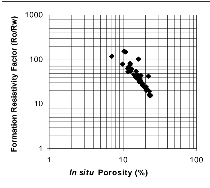
FIGURE 2.10. Cross-plot of in situ formation electrical resistivity factor versus in situ porosity.
