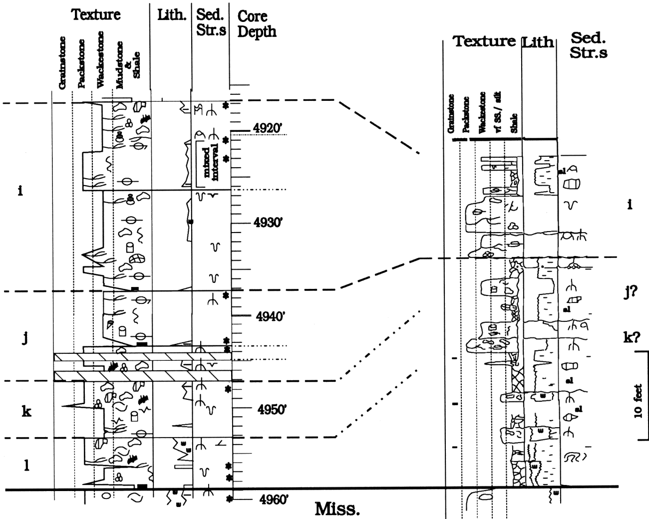
FIGURE 28—COMPARISON OF MID-SHELF SEQUENCES i , j , and k , in Gray County to possible proximal equivalents preserved within incised valley in Clark County. Well locations in fig. 2 and key in fig. 27.
