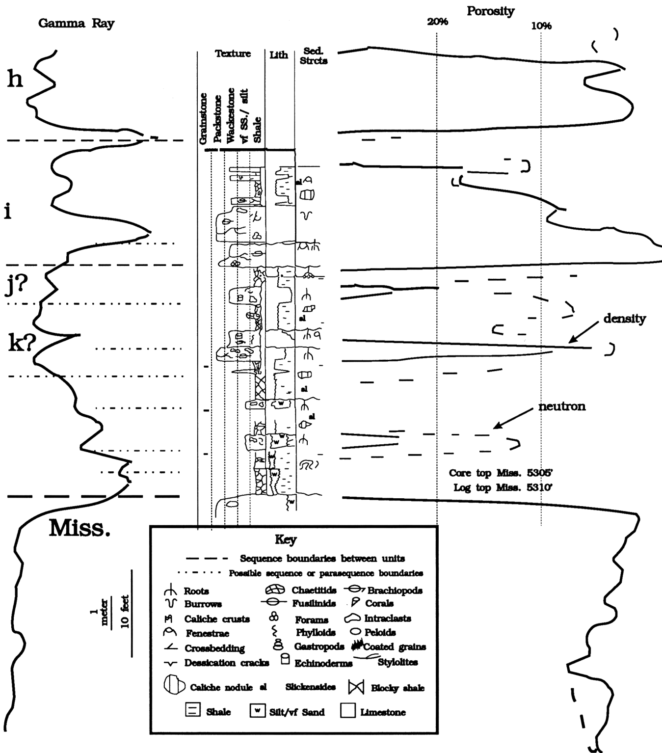
FIGURE 27—CORE DESCRIPTION AND WIRELINE LOG OF LOWER "GRAY GROUP" SEQUENCES IN THE LADD #1 HARRIS, FORD COUNTY. Core depths were adjusted down 5 ft to match log depths.
