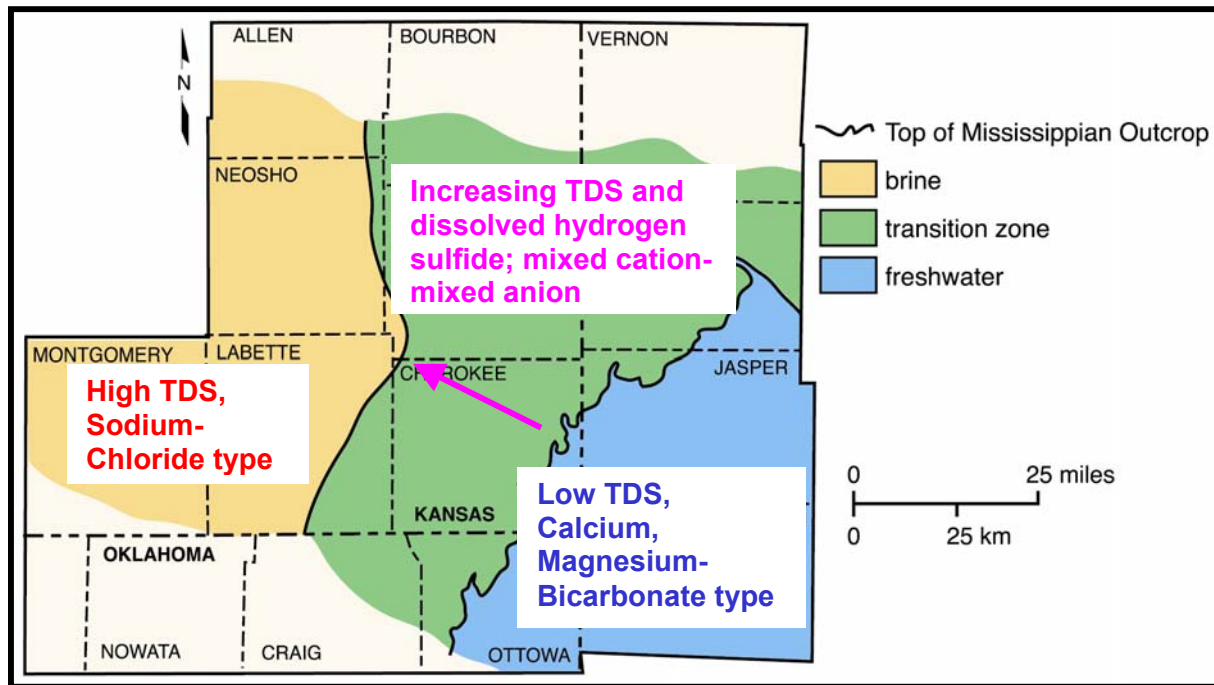
Figure 4. General characterization of ground-water quality in the Ozark aquifer in southeast Kansas, southwest Missouri, and northeast Oklahoma. Taken from Macfarlane and Hathaway (1987).
