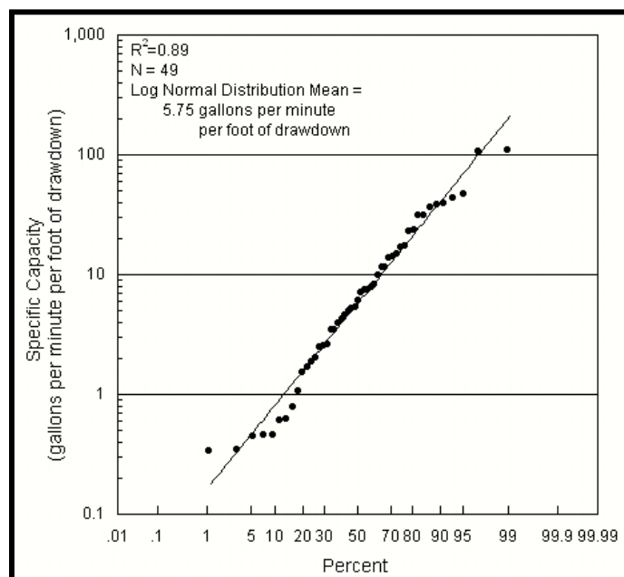
Figure 10. Specific capacities calculated from production tests of wells tapping the Ozark aquifer in southeast Kansas, southwest Missouri, and northeast Oklahoma.
