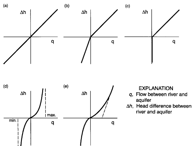
Fig. 3 Illustrations of the various mechanisms describing flow between the river and aquifer ( q ) as a function of the difference between the river and aquifer heads ( \Delta h ). a–d represent various flow conditions; see text for additional explanations. (Adapted from Rushton and Tomlinson 1979)
