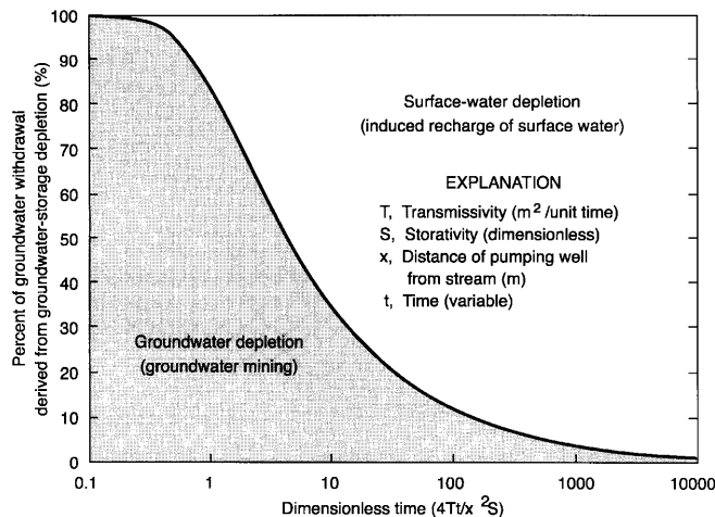
Fig. 9 Transition from reliance upon groundwater storage to induced recharge of surface water. (Adapted from Balleau 1988)
